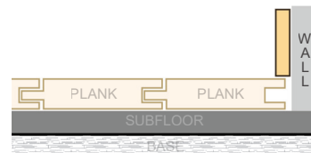
Wall Base
